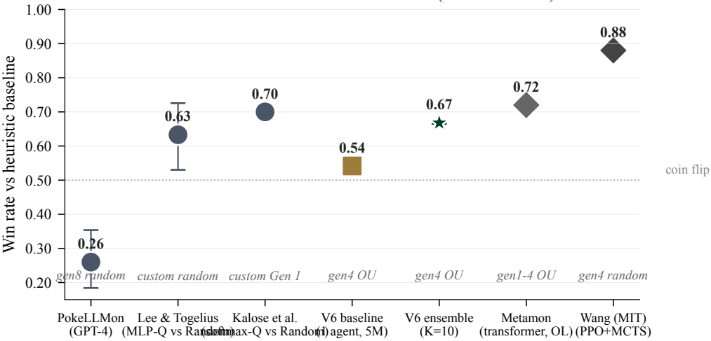
Pokemon-RL results vs heuristic baseline (format in italics )
